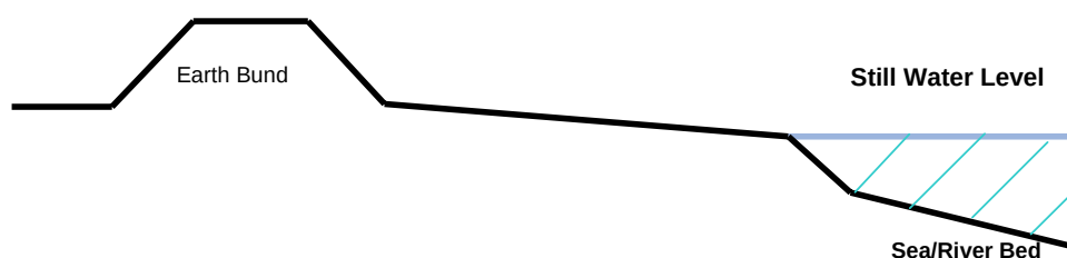
FIGURE 5-1 TYPICAL CROSS SECTION OF EARTH BUND
